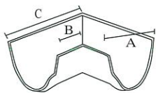
Angle 90° join in RSD03E
